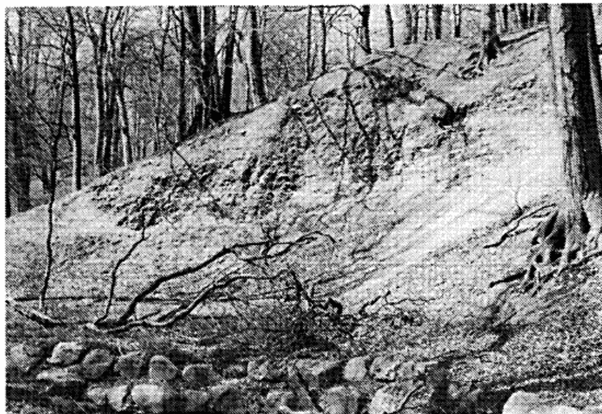
Fig. 9. A little niche in the Pálsjö valley with a strong, mechanically weathering of the shale.
