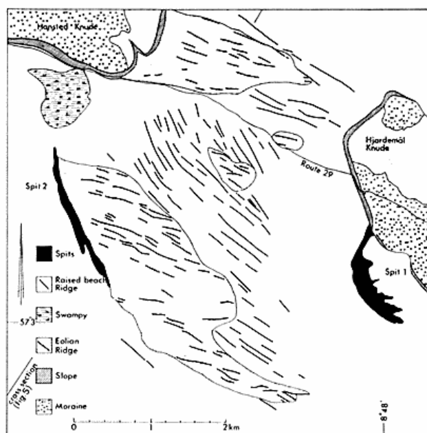
Fig. 6. Morphological lineaments and interpretation following Christiansen & Bowman (1986).
