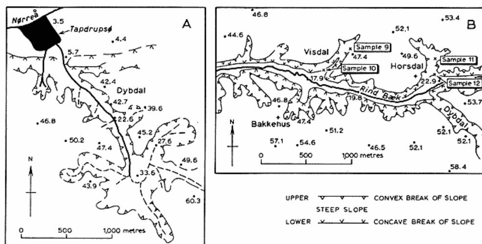
Fig. 6a. Morphological diagram of Dybdal, one of the longer tributary valleys draining north into Nørreå, on the north side of Vinkel parish.
