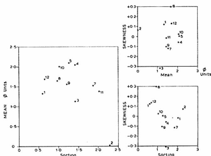
Fig. 3. Graphs illustrating the relationship between sedimentary parameters.
