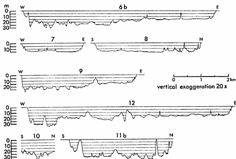
Fig. 3. Echo-sounded profiles from the lagoon of Nukuria. Vertical distance between lines = 5 m (15 ft.) For positions: see fig. 2.
