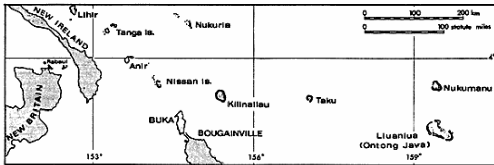
Fig. 1. Position of the four atolls, Nukuria, Kilinailau, Taku and Nukumanu. While Nissan is an elevated atoll, Lihir, Tanga and Anir are of volcanic origin.
