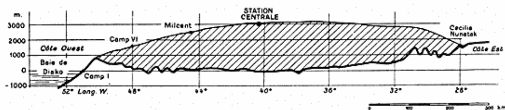
Fig. 3. Cross section through the Ice Cap from Disko Bugt to Cecilia Nunatak (Exp. Pol. Franc., Rapp. prélim. 16, 1953).
